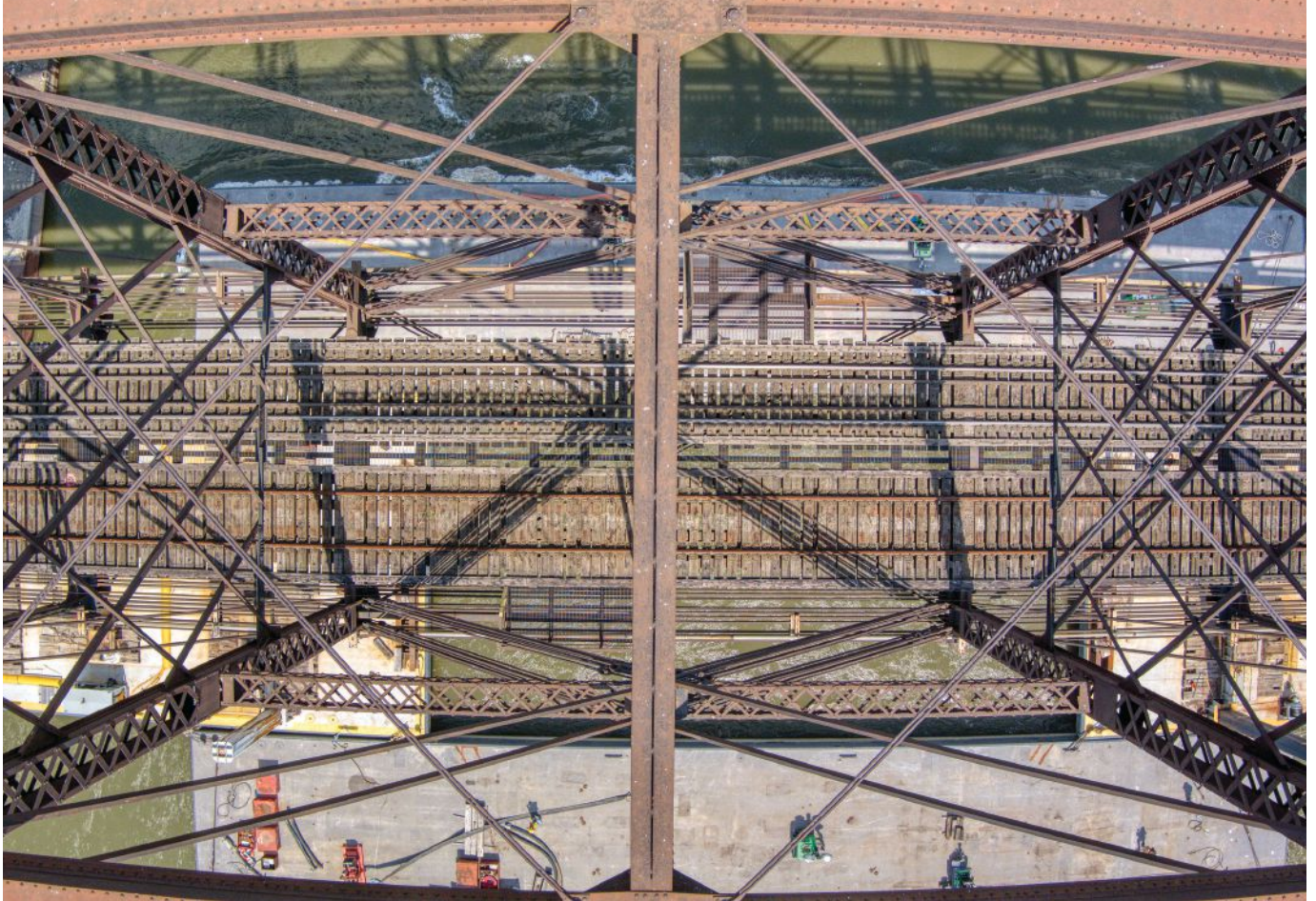
Key aspects of the span change-out included strengthening the existing truss chords for removal, strengthening the existing piers for the gantry system, placing the gantry system for lifting and sliding the spans, and maintaining barge stability and maneuverability in and around obstacles in the river while positioning the truss under the gantry system.
