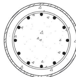
Fig. 2. Group 1 example: encased and filled composite column in composite frame construction.
