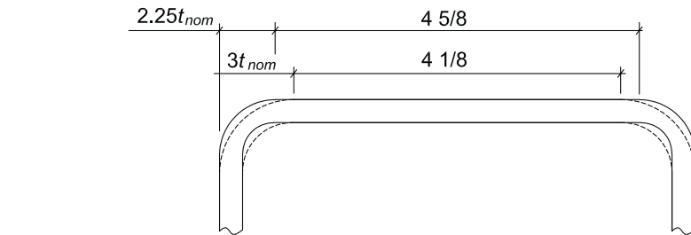
Fig. 1. Corner radii dimensions for square HSS (flat dimensions for HSS6×6× 5 / 16 ).
