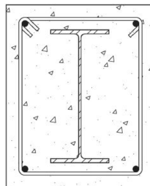
Fig. 3. Group 2 example: steel floor beam wrapped in concrete.
